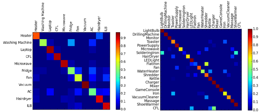
Figure 4: The confusion matrix of the PLAID (left) and WHITED (right) dataset when classified using n = 50 and f = 50 . The rows are the real labels of the appliance and the columns the predicted labels.
