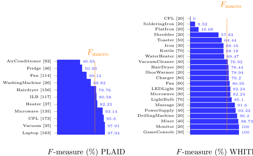
Figure 3: The F -measure per appliance for the PLAID (left) and WHITED (right) dataset of the CNN for n = 50 and f = 50 . The number of appliances per type are mentioned between the brackets. (CFL = compact fluorescent lamp, ILB = incandescent light bulb)
