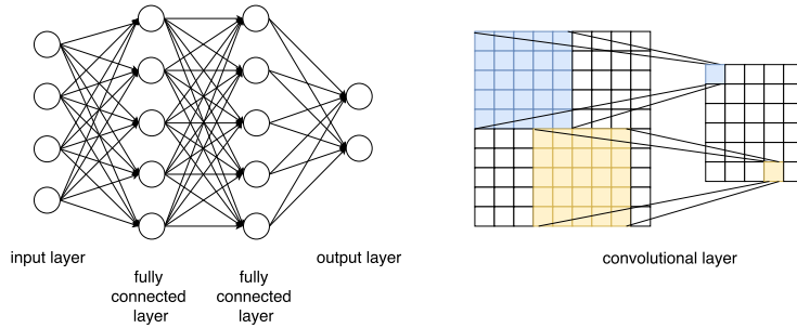
Figure 2: (left) a NN consisting of an input layer, two fully connected layers and an output layer, (right) a convolutional layer.
