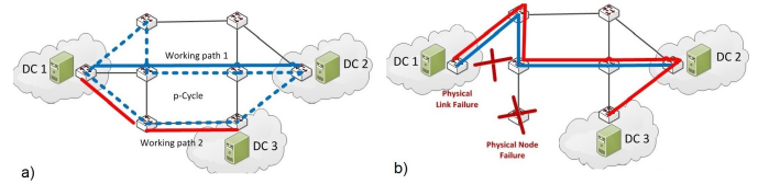
Fig. 8. Example of a p-Cycle. a) FIPP p-Cycle (dotted line) used to protect two working paths. b) Example of double failures and the use of p-Cycle for recovery.
